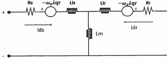
Figure 2. D-axis equivalent circuit
