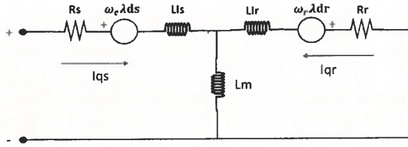
Figure 1. Q-axis equivalent circuit
