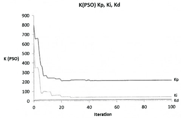
Figure 10. PID gains obtained from PSO
