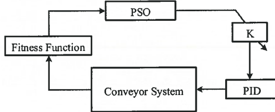
Figure 9. Diagram of PSO based PID controller.
